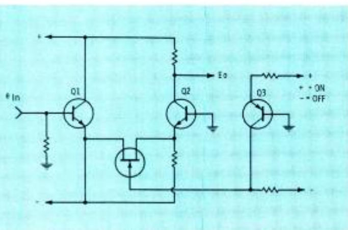
Fig. 5 Squelch amplifier.
