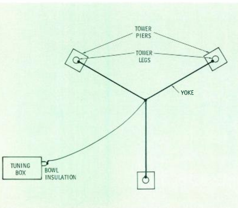
Fig. 1 The KFGO pattern. The solid dots represent the original FCC Monitor Point Bearings.
