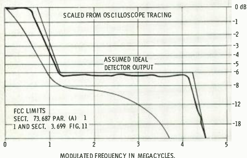
Fig. 2 Tracing from oscilloscope of the diode response curve.
