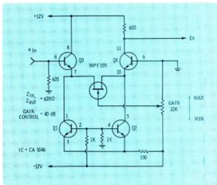
Fig. 6 Practical example of an attenuator.
