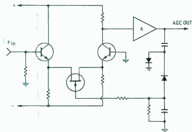
Fig. 4 A range compressor, another AGC device.
