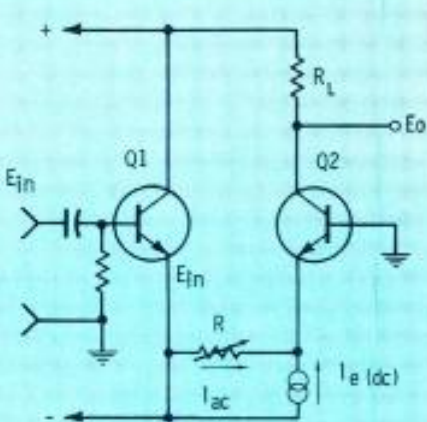
Fig. 2 Schematic of a gain controlled amplifier.
